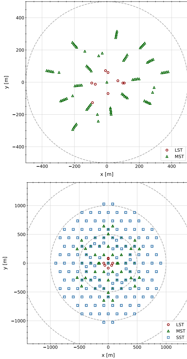
Figure 1: Simulated telescope positions within the third large-scale MC production (see section 2 for details). Top: La Palma telescope positions including all radially-scaled MST layouts. The available positions are restricted by the site topography, buildings and roads. Bottom: Paranal telescope positions before applying any radially-symmetric transformation (scaling number 1). LST positions are indicated by red circles, MSTs by green triangles, and SSTs by blue squares.
